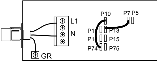
Figure 6.0d 230V 50Hz Wiring
