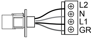
Figure 6.0d 230V 50Hz Wiring
